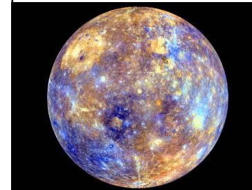
Mercury
